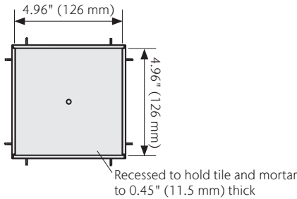
6" Tile-In Grate
