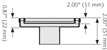
Threaded Adapter
